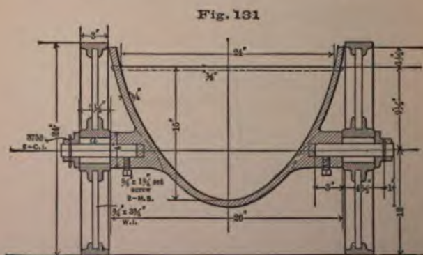
SLAG-POT WITH ROLLER BEARINGS.
